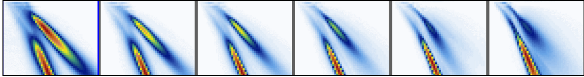
Figure 9: Beam deformation with increasing gap between wedge and surface
