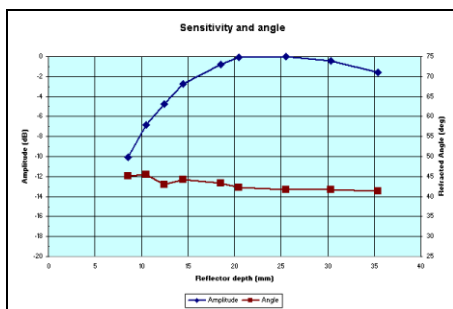
Figures 8a and 8b: beam characteristics graphs
