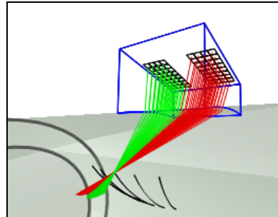
Figure 7: angle and focal point
