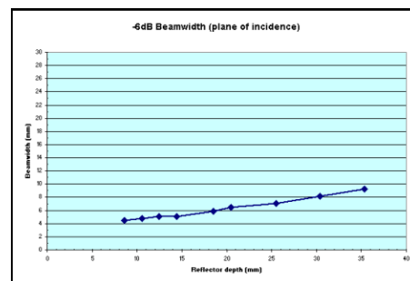
Figures 8a and 8b: beam characteristics graphs
