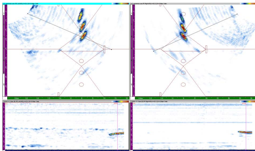
Figure 10: image of one-line scan with TRL PA probes
