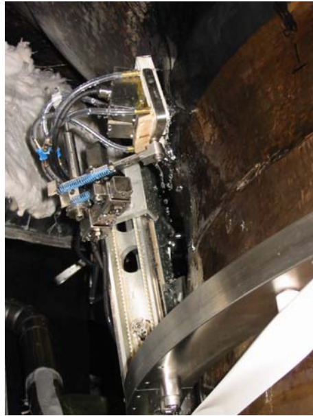
Figure 12: TRL PA probe on MCP weld
